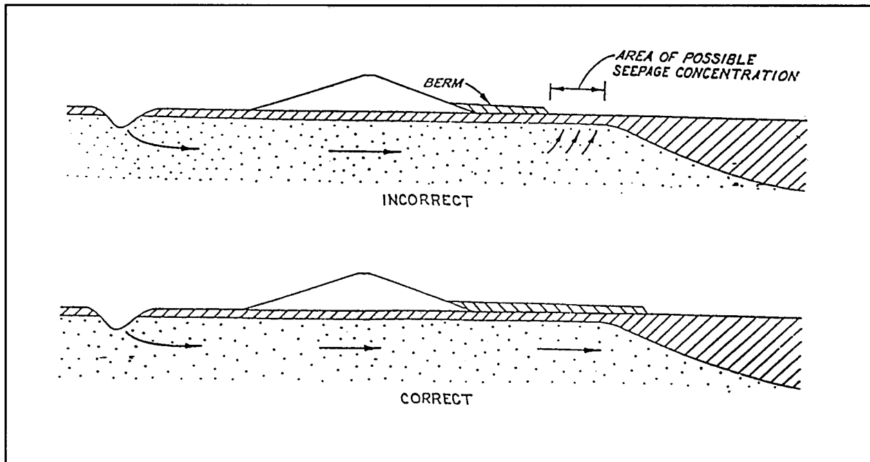
Figure 5-1. Example of incorrect and correct berm length according to existing foundation conditions
